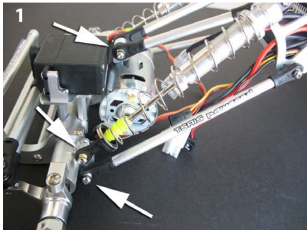
1 Front axle: Install the links and shocks to the designated positions on the front axle as shown.
