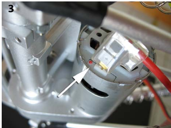
3 CAUTION: the motor +/- terminals are soft, so use extra caution when connecting the wires. Front motor: Red (+) wire connects to the terminal that is marked red and the black (-) wire connects to the other terminal. Rear motor: Black (-) wire connects to the terminal that is marked red and red wire connects to the other terminal (opposite of the front).
