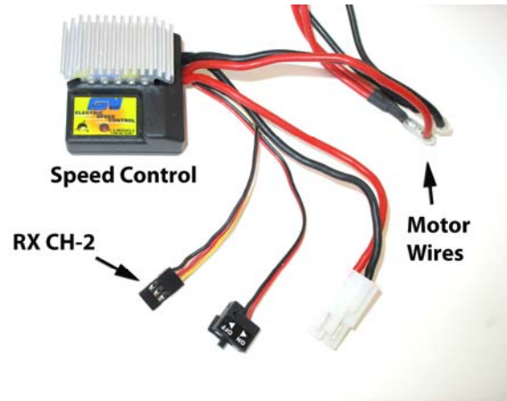
Speed control: it has been installed onto the lower deck of the chassis, so plug the RX CH-2 plug into the receiver CH2 hole, connect the motor wires, and then attach the on-off switch onto the chassis side plate with double sided tape.
