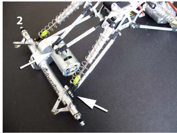
2 Rear axle: Install the links and shocks to designated positions on the rear axles as shown.
