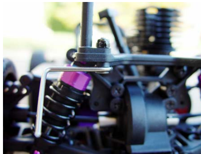
Install the body post plate back onto the shock tower.
