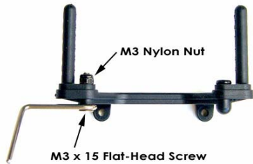
Install the wire with the M3 x 15mm flat-head screw and nylon nut.
