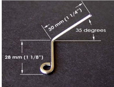
Bend the wire as shown.
