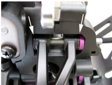
<Fig. 1> Savage X ONLY: Install the black M4x10 washers (see arrows) on the front and rear of the suspension arms before you insert the pin.
